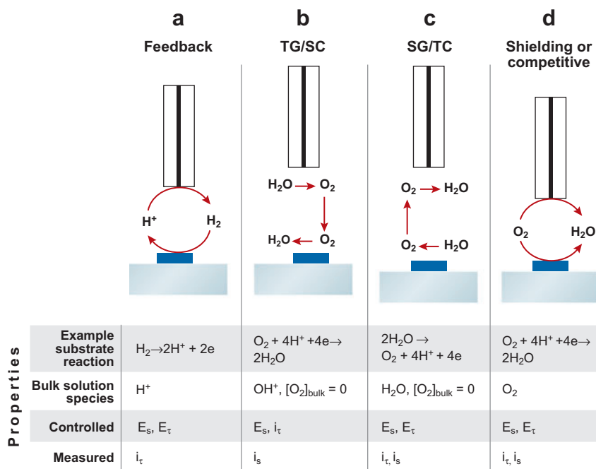
Figure 10 Schematic representation of different modes of substrate screening in scanning electrochemical microscopy. TG, tip generation; SC, substrate collection.
